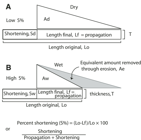
Figure 2. Idealized critically tapered wedges for dry (A) and wet (B) orogen. Area of the wedge, A_d (dry) A_w (wet), is function of thickness of undeformed strata ( T ), amount of shortening ( S ), and amount of propagation (length final). A_e is the amount of material that has been removed from the wet wedge.
